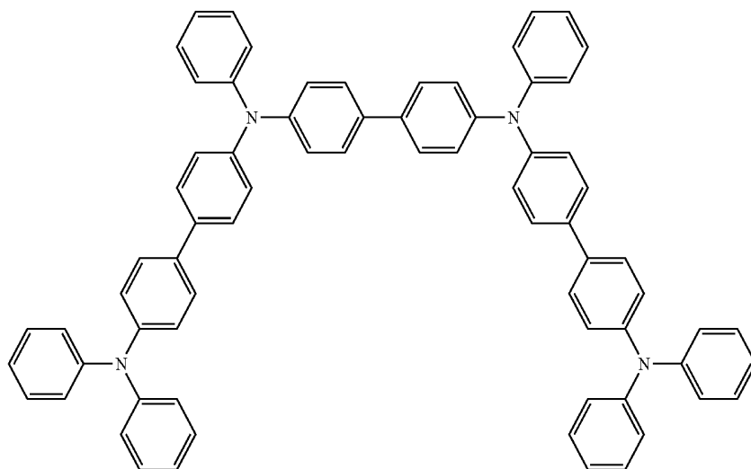
[Compound 100]
