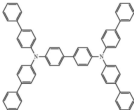
Compound 102]
