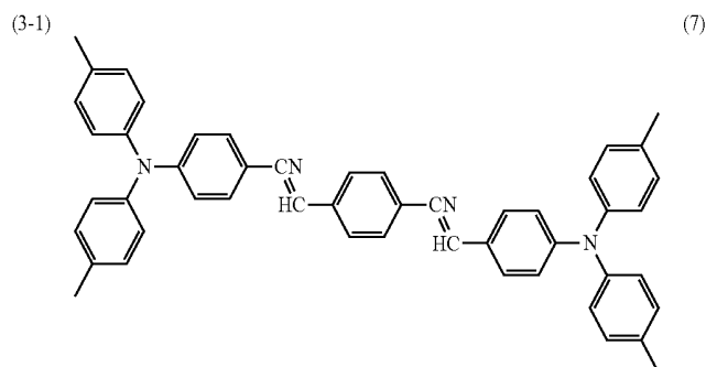
[Compound 87]
