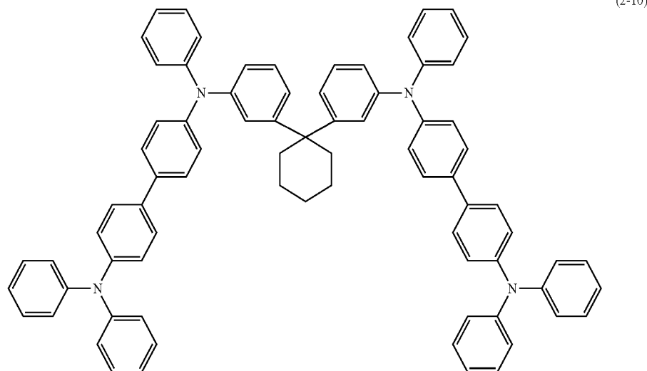
[Compound 109]
