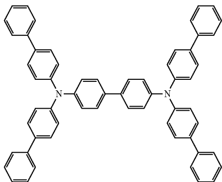
Compound 88]
