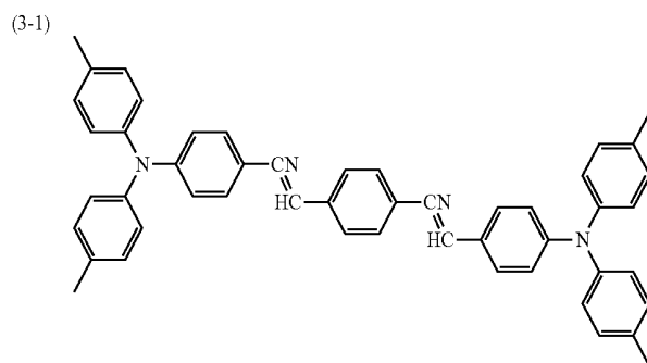
[Compound 101]
